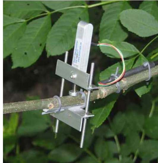
Figure: Ecomatik DD-S sensor (stem)
